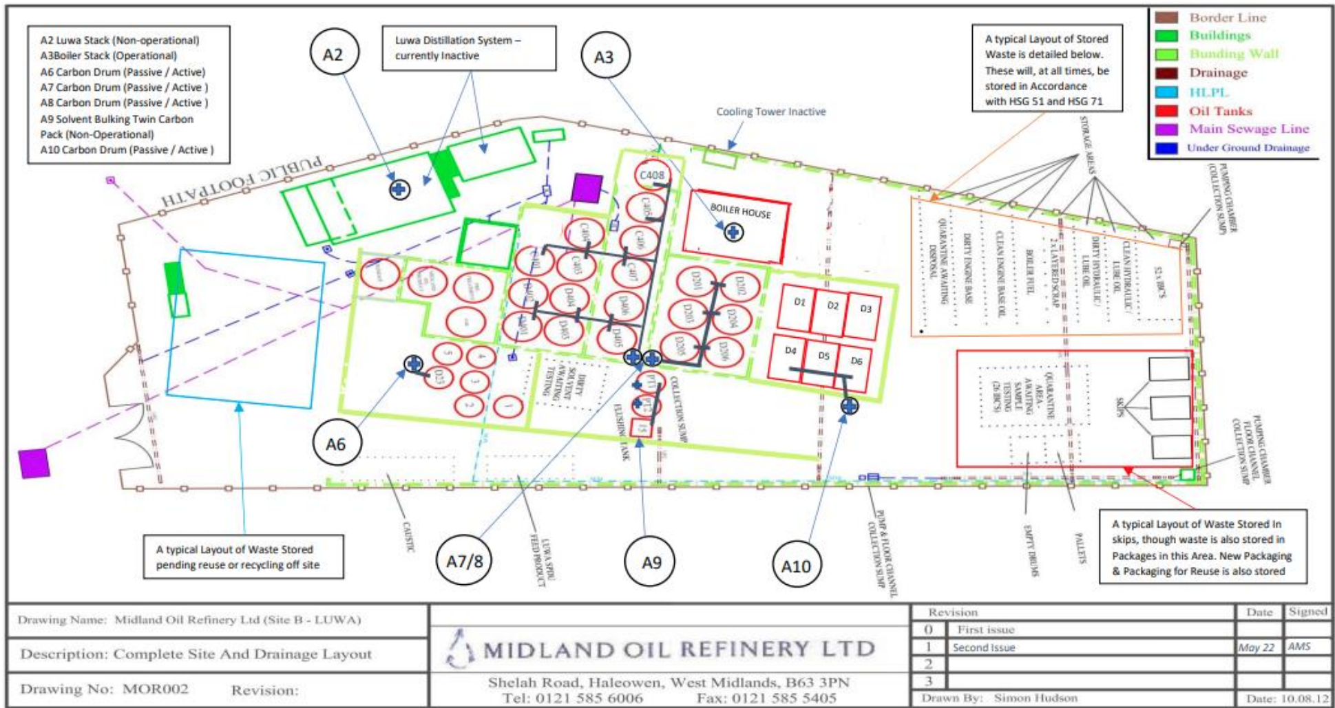
Figure 2b: Site Layout Plan including emission points (Site B –LUWA)
