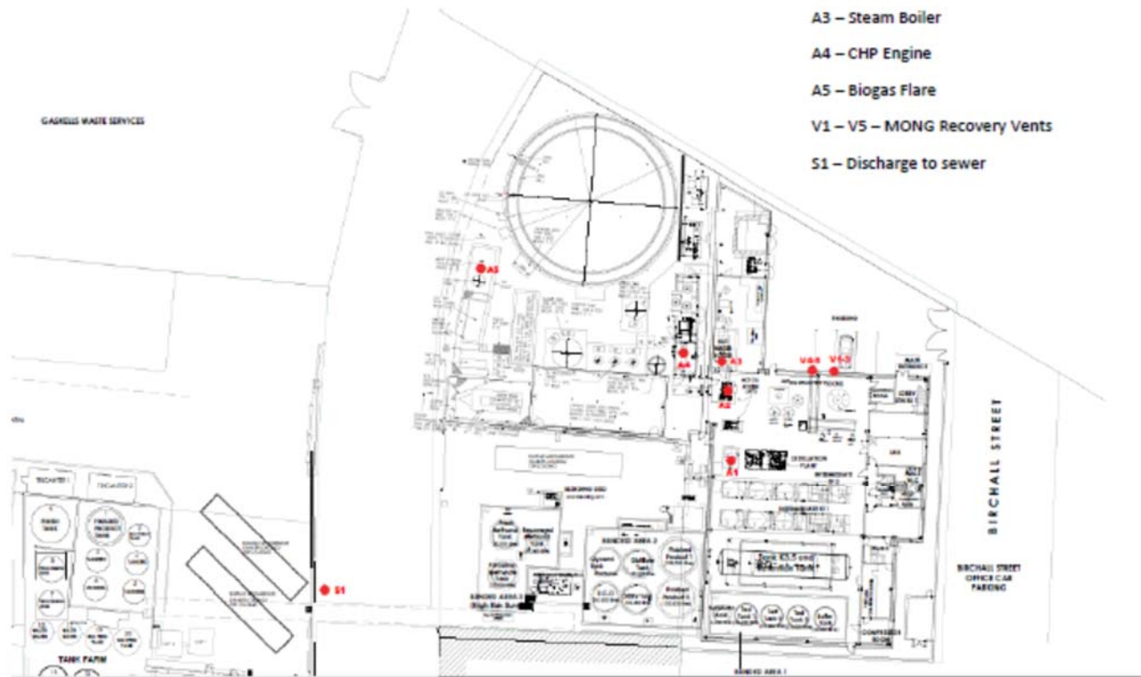
Figure 3A – Site Layout Showing Emission Points Olleco Liverpool – Birchall Street Biodiesel and AD Plant
