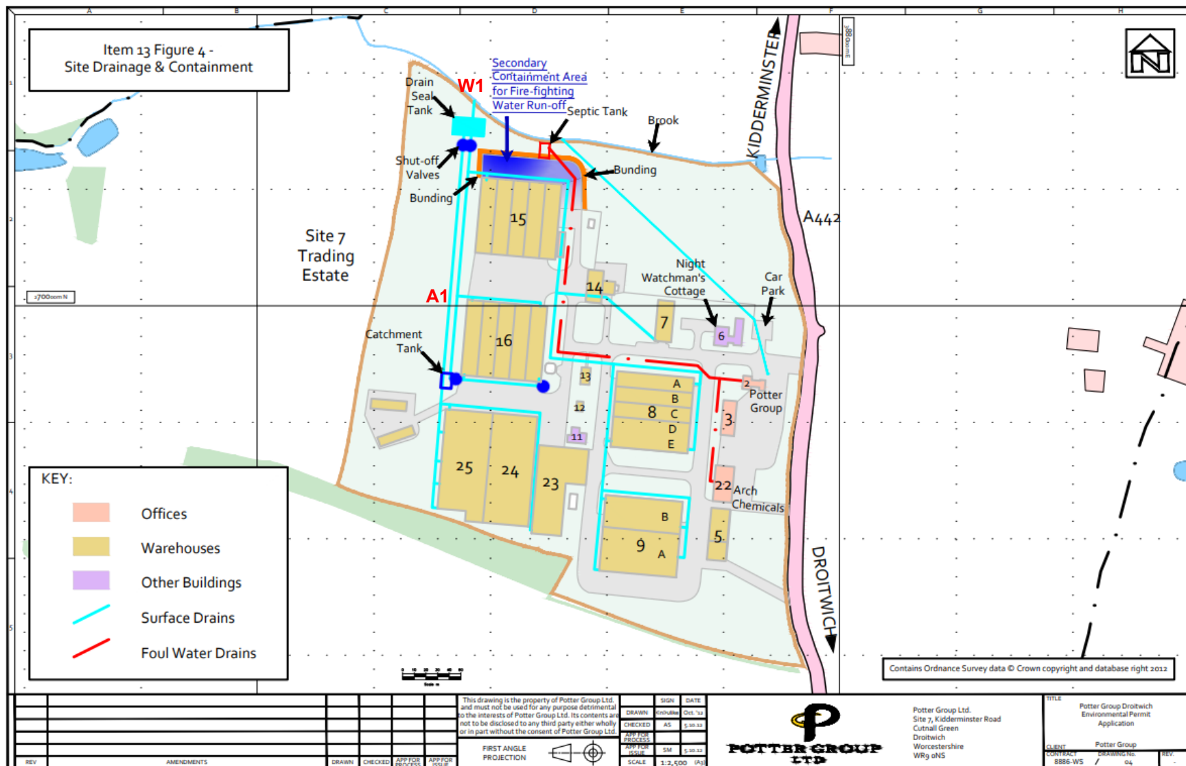
Figure 3: Site Layout Plan including emission points
