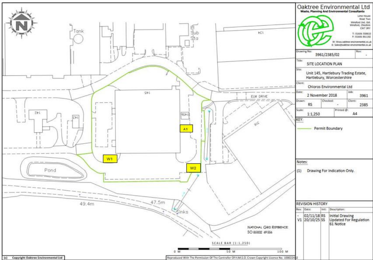
Figure 1: Site location with emission points and permit boundary
